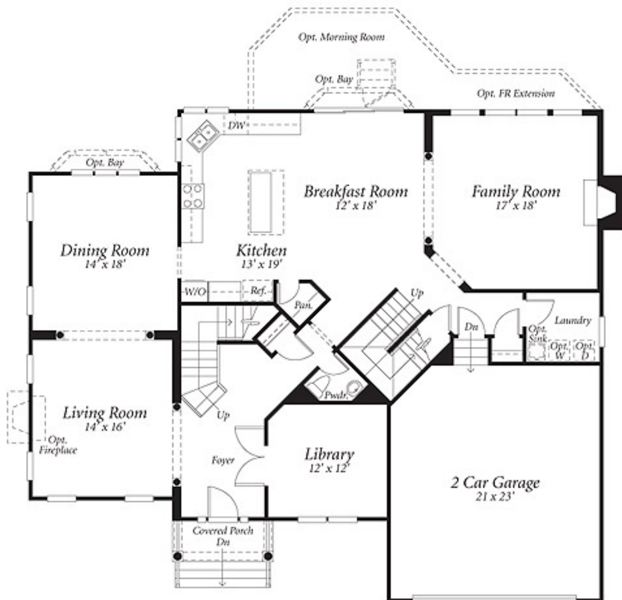
FIRST FLOOR
